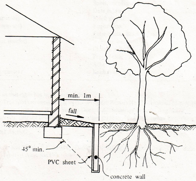
Cut off wall
