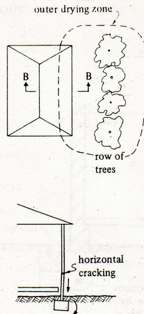
SECTION B
