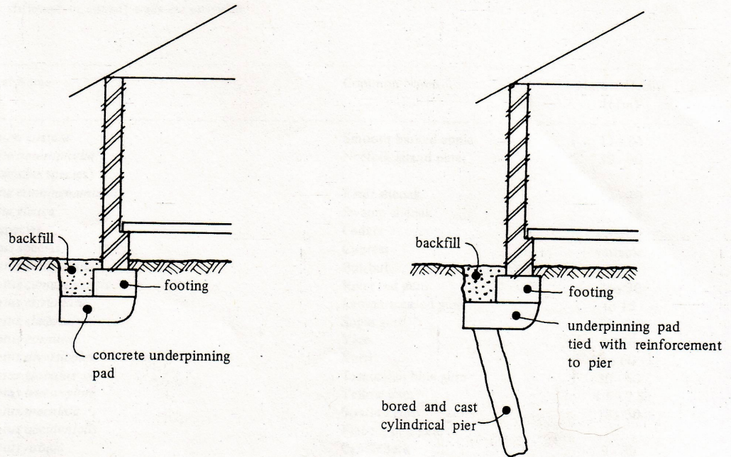
Underpinning
